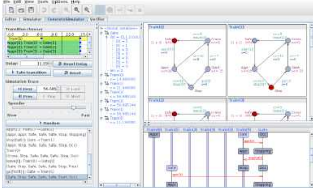
Figure 15: The concrete simulator in UPPAAL.
