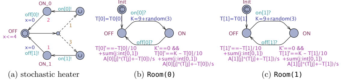
Figure 10: A simple two room example with an autonomous heater
